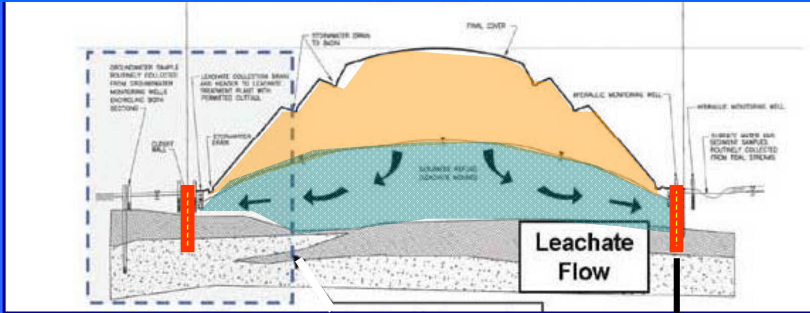
Leachate Containment Wall
